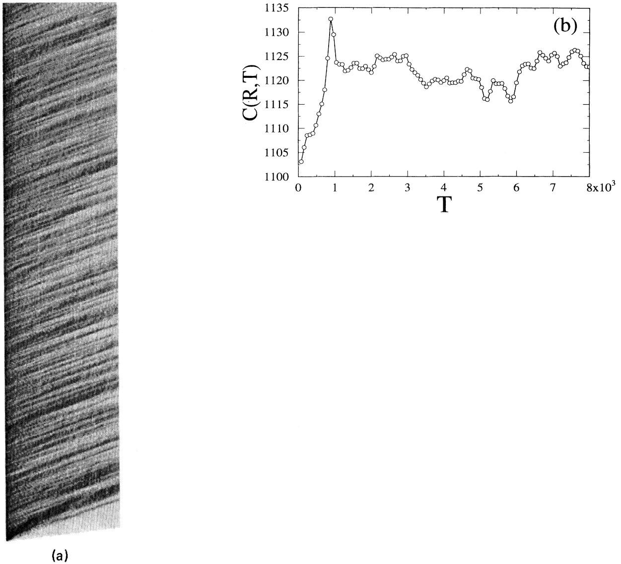
FIG. 11. (a) Time evolution of the density n_i \{i=1,2,\dots,100\} in 100 bins in the pipe of L=1000 , W=5 , and I=0.5 . Other model parameters are p=0.5 , b=0.5 , and g=0.2 . Densities at a given time are plotted from left to right (the direction of gravity), while densities at different time steps are plotted from bottom to top (the direction of time increase). Time goes from 0 to 40 000 time steps. The gray scale of each bin is a linear function of n_i . Darker regions correspond to higher densities, (b) Two-point density-density correlation function C(R, T) versus the time difference T (in time step) at a fixed spatial separation R=30 for the evolution shown in (a).
