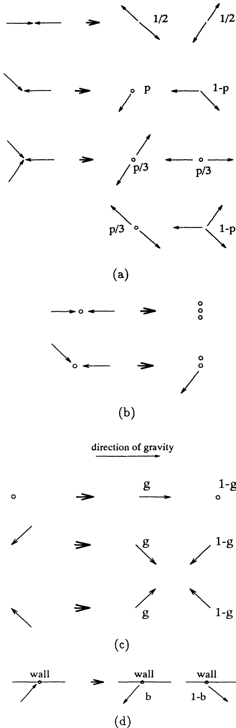
FIG. 1. (a) Probabilistic collision rules for two- and three-body collisions. Thin arrows represent particles and small circles stand for rest particles. The number next to a configuration is the probability that the configuration takes place. (b) Collision rules for moving particles with a rest particle. Immediately after the collision, more than one rest particle on a site will hop to the nearest-neighbor sites randomly until they find a suitable site with no rest particle already there. (c) Gravity may change the momentum of the particle by a unit vector in the direction of gravity. (d) Collision rule for a moving particle colliding with the wall.
